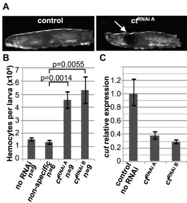
Figure 5. Haploinsufficiency of the D melanogaster CUX1 homologue, cut , leads to melanotic tumor formation and hemocyte hyperproliferation in vivo. cut knockdown was performed by crossing flies expressing ct RNAi in a construct containing a UAS promoter and GFP tag with flies expressing the GAL4 driver under the hemocyte-specific hml promoter. Two different ct targeting constructs were tested: ct RNAi A and ct RNAi B . (A) ct RNAi A but not wild-type ( w 1118 ; hml -GAL,UAS-GFP/+), Drosophila third instar larvae develop melanotic tumors (indicated by the arrow). (B) cut knockdown leads to increased numbers of hemocytes. Circulating hemocytes bled from wild-type, nonspecific RNAi, ct RNAi A , and ct RNAi B developing larvae were stained with Hoechst and quantified (mean \pm SEM). (C) Haploinsufficient levels of cut are confirmed by quantitative RT-PCR of cut from hemocyte RNA. One representative experiment of 3 is shown.
