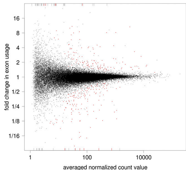
Figure 4. Fold changes of exon usage versus averaged normalized count value for all tested counting bins for the Brooks et al. data. (Red) Significance at 10% FDR. Bars at the margin represent bins with fold changes outside the plotting range.
