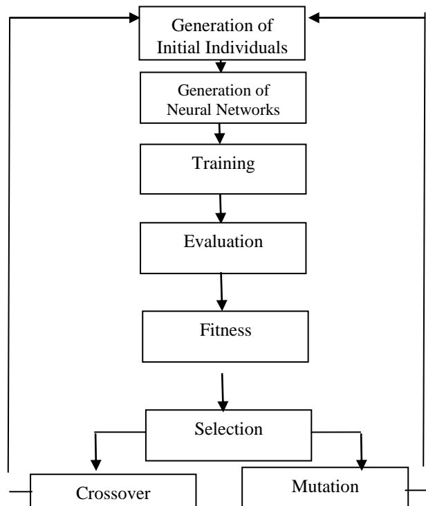
Principle Structure of GA and GANN System
