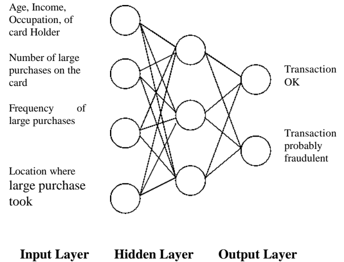
Fig. 2: Layer of Neural Network in Credit Card
