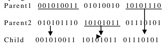
Figure6: Two-point crossover
