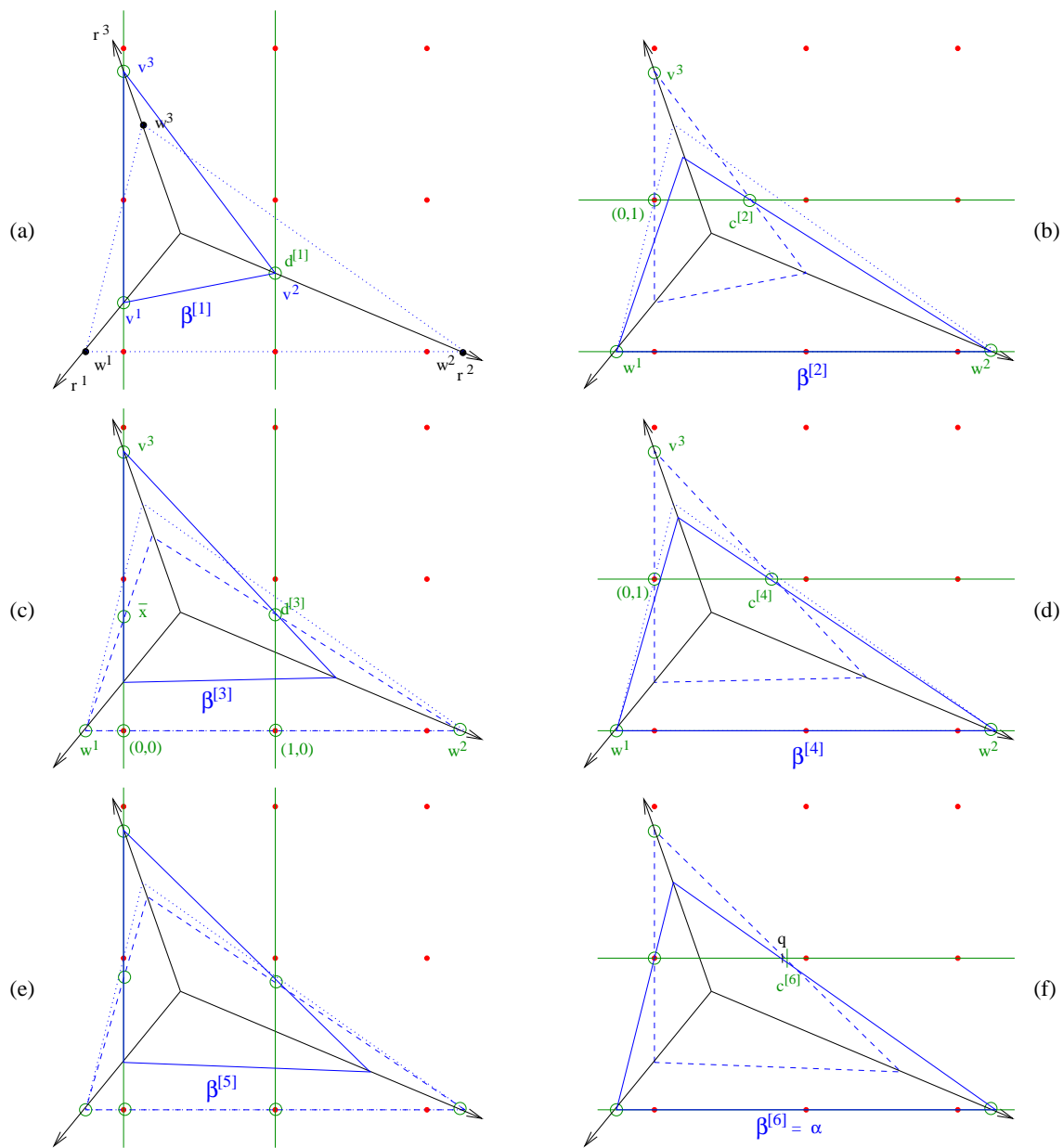
Figure 5: In each frame, the dotted triangle is L_\alpha . The dashed triangle is the induced lattice-free set of the inequality obtained in the previous step. The circles are the x -vertices obtained by the application of the disjunction. The solid triangle is the induced lattice-free set of the inequality that is valid for these x -vertices.
