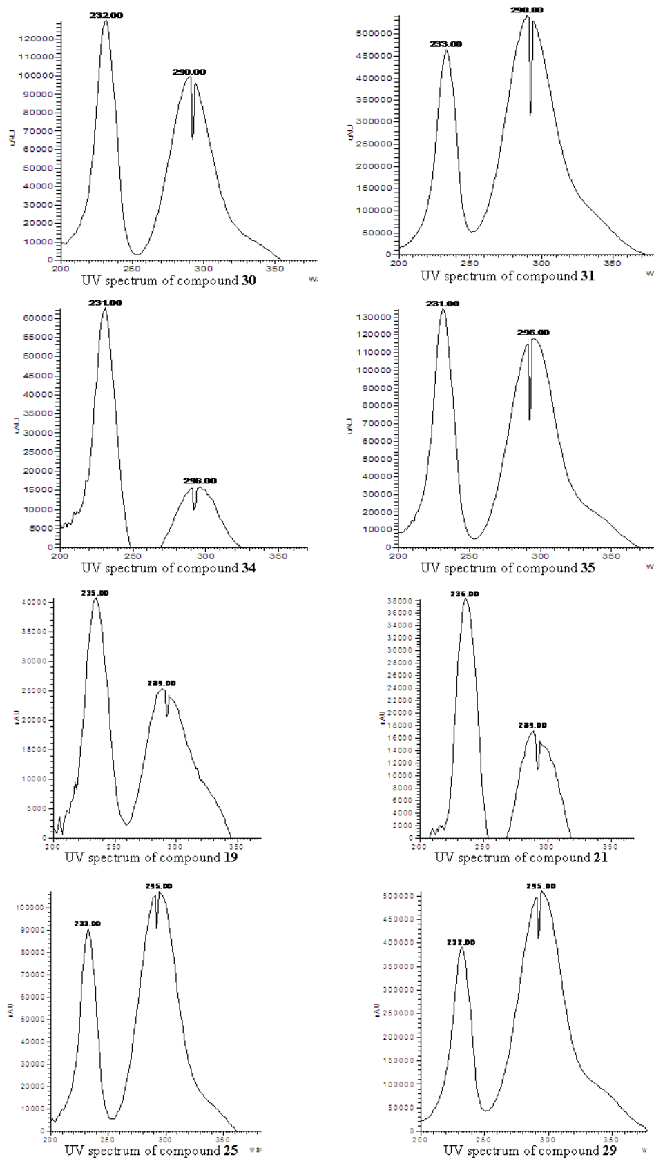
Figure S2. UV spectra of compounds 30 , 31 , 34 , 35 and 19 , 21 , 25 , 29 .
