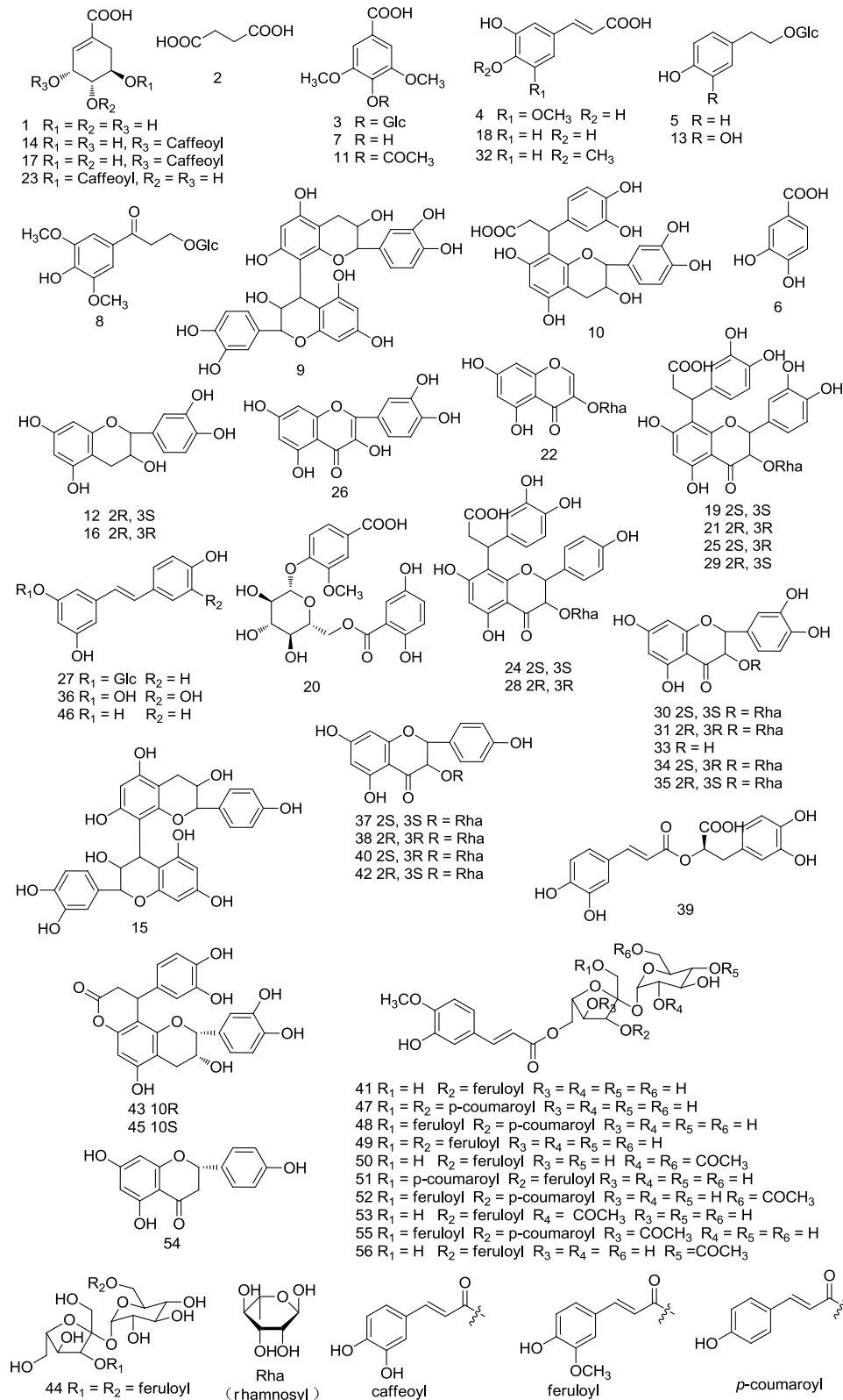
Figure S1. The chemical structures of identified compounds of Smilacis glabrae extract.
