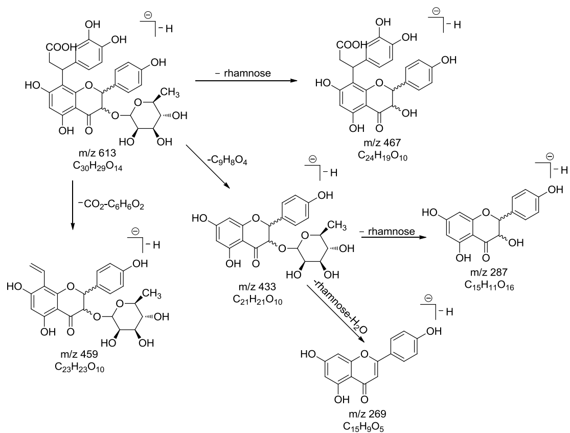
Figure S3. Proposed fragmentation pathway for compounds 24 and 28 .
