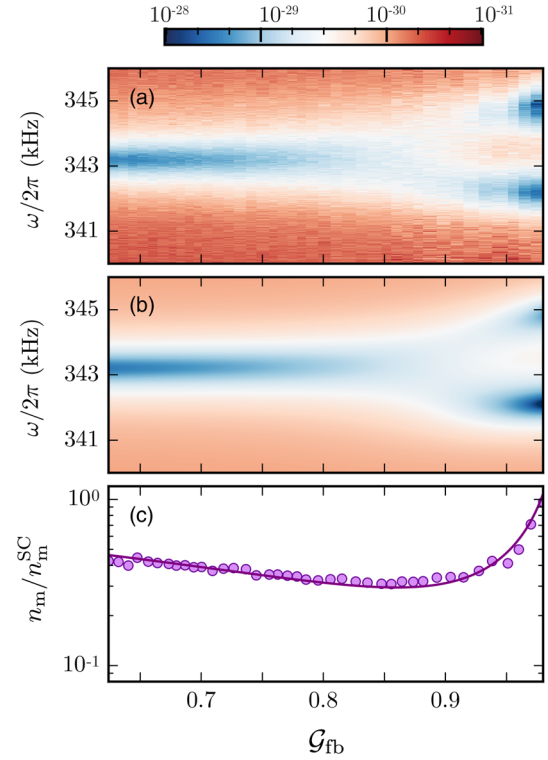
FIG. 4. Transition between the weak- and strong coupling regime. (a) Power spectra of mechanical displacement fluctuations varying the feedback gain \mathcal{G}_{\text{fb}} , and (b) the corresponding simulation evaluated as S_{xx}(\omega) = x_0^2 S_{qq}(\omega) with x_0 = \sqrt{\hbar/2m\omega_m} . The color scale is shown at the top in \text{m}^2/\text{Hz} . At low gain the mechanical motion is described by a single mode, the dynamics of which is modified by the in-loop optomechanical interaction. At high gain, instead, the spectrum becomes double-peaked: the strong interaction produces hybridized optomechanical modes and the mechanical motion is a superposition of these two normal modes. The difference in frequency between the two peaks in the spectrum with maximum gain corresponds to G = 2\pi \times 1.87 \text{ kHz} . The parameters for this measurement ( P , \Delta , \kappa and g_0 ) yield G = 2\pi \times 1.96 \text{ kHz} , in good agreement with the experimental estimation. (c) The ratio of the effective phonon number with and without feedback. The circles are obtained by numerical integration of the measured spectra, while the solid line corresponds to Eq. (5), evaluated using the measured parameters, which is valid both in the weak- and in the strong coupling regime. The feedback scheme enhances the cooling rate with respect to standard sideband cooling by a factor of 5 dB.
