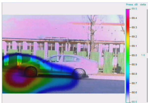
Fig. 2. Noise emissions of Škoda Octavia 1.4 (gear engaged 4, speed 50 km/h)
