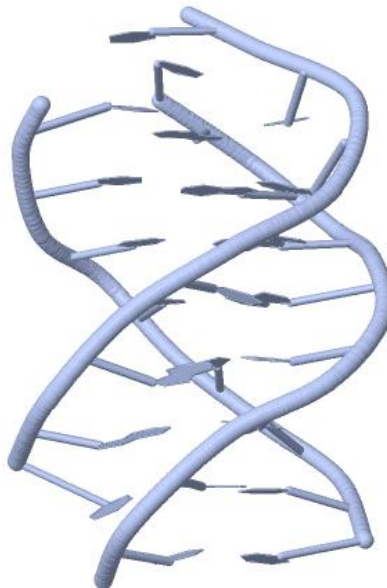
FIGURE 1. Cartoon of 3D structure of a purine-purine-pyrimidine DNA triplex containing G-GC and T-AT triples. This picture is a snapshot of the structure with the identifier 134D obtained from the Protein Data Bank. The structure was resolved using a combined NMR and molecular dynamics approach by Radhakrishnan and Patel[35].
