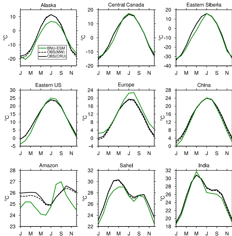
Fig. 1. Climatological annual cycle of 2 m air temperature for selected regions for BNU-ESM and two observational estimates for the period 1976–2005. MW denotes version 2.01, 0.5^\circ \times 0.5^\circ monthly time series from Matsuura and Willmott (2009a). CRU is the Climatic Research Unit 0.5^\circ \times 0.5^\circ TS 3.1 dataset (Harris et al., 2013). Regions are defined as follows: Alaska ( 56\text{--}75^\circ\text{N} , 167\text{--}141^\circ\text{W} ), Central Canada ( 46\text{--}61^\circ\text{N} , 123\text{--}97^\circ\text{W} ), Eastern Siberia ( 51\text{--}66^\circ\text{N} , 112\text{--}138^\circ\text{E} ), eastern United States ( 27\text{--}47^\circ\text{N} , 92\text{--}72^\circ\text{W} ), Europe ( 37\text{--}57^\circ\text{N} , 0\text{--}32^\circ\text{E} ), China ( 18\text{--}42^\circ\text{N} , 100\text{--}125^\circ\text{E} ), Amazon ( 14^\circ\text{S}\text{--}5^\circ\text{N} , 74\text{--}53^\circ\text{W} ), Sahel ( 4\text{--}19^\circ\text{N} , 0\text{--}32^\circ\text{E} ), and India ( 4\text{--}28^\circ\text{N} , 68\text{--}94^\circ\text{E} ).
