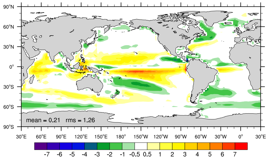
Fig. 4. Annual mean precipitation differences ( \text{mm day}^{-1} ) of BNU-ESM relative to the GPCP climatology for the period 1979–2005.
