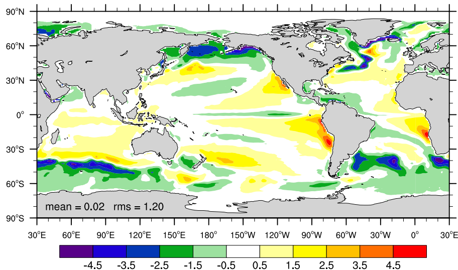
Fig. 3. Annual mean SST differences ( ^{\circ}\text{C} ) of BNU-ESM relative to the 1^{\circ} \times 1^{\circ} estimates from the Hadley Center Sea Ice and SST (HadISST) data set (Rayner et al., 2003) for the period 1976–2005.
