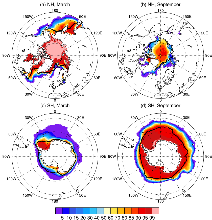
Fig. 6. Mean sea ice concentration (%) over years 1976–2005 of the BNU-ESM historical run for both hemispheres and for March (a, c) and September (b, d). The solid black lines show the 15% mean sea ice concentration from SSM/I observations (Comiso, 1999).
