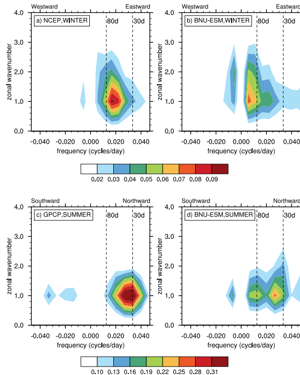
Fig. 9. November–April wavenumber–frequency spectra of 10^{\circ}\text{S} – 10^{\circ}\text{N} averaged daily zonal 850 hPa winds NCEP observation (a) and BNU-ESM (b) . May–September wavenumber–frequency spectra of 15^{\circ}\text{S} – 30^{\circ}\text{N} , 65 – 95^{\circ}\text{E} averaged daily precipitation for GPCP observation (c) and BNU-ESM (d) . Individual spectra were calculated for each year and then averaged over all years of data. Only the climatological seasonal cycle and time mean for each November–April or May–September segment were removed before calculation of the spectra. The averaging period is 1980–2005 for BNU-ESM historical run, and 1997–2006 for observations.
