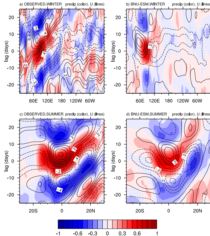
Fig. 8. November–April lag-longitude diagram of 10^{\circ}\text{S} – 10^{\circ}\text{N} averaged intraseasonal precipitation anomalies (colors) and intraseasonal 850 hPa zonal wind anomalies (contours) correlated against intraseasonal precipitation in the Indian Ocean reference region ( 10^{\circ}\text{S} – 5^{\circ}\text{N} , 75 – 100^{\circ}\text{E} ) for NCEP observation (a) and BNU-ESM (b) . May–September lag-latitude diagram of 65 – 95^{\circ}\text{E} averaged intraseasonal precipitation anomalies (colors) and intraseasonal 850 hPa zonal wind anomalies (contours) correlated against intraseasonal precipitation at the Indian Ocean reference region for NCEP observation (c) and BNU-ESM (d) . The averaging period is 1980–2005 for BNU-ESM historical run, and 1997–2006 for observations.
