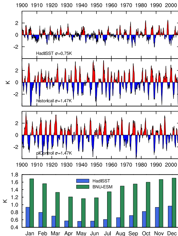
Fig. 10. Time series of detrended monthly SST anomalies of the Niño-3.4 region ( 5^{\circ}\text{S} – 5^{\circ}\text{N} , 170^{\circ}\text{W} – 120^{\circ}\text{W} ) from HadISST, the BNU-ESM historical and piControl runs. The anomalies are found by subtracting the monthly means for the whole time series. The bottom sub-figure is standard deviation of monthly Niño-3.4 SST anomalies from HadISST and the BNU-ESM historical run.
