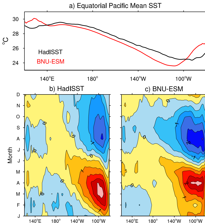
Fig. 5. Mean SST (°C) along the equator in the Pacific Ocean (a) and annual cycle of SST anomalies for the period of 1976–2005 from HadISST (b) and the BNU-ESM historical run (c) .
