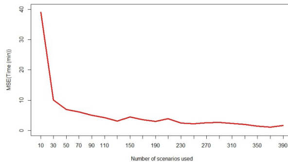
Figure 4: Evolution of the mean square sizing error with the number of scenarios considered in the simulation. Error is expressed in extra minutes of overshoot. Objective overshoot time ( T ): 19 minutes.
