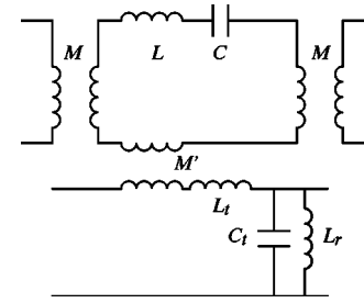
FIG. 4. Equivalent circuit for a transmission line loaded with metal rods and SRRs.
