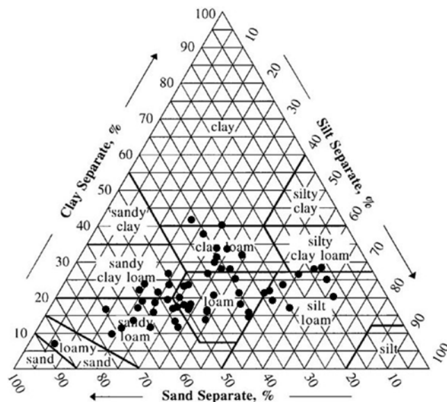
Fig. 3. Soil texture of 0- to 10-cm depth of 57 field trials on tall fescue pasture.
