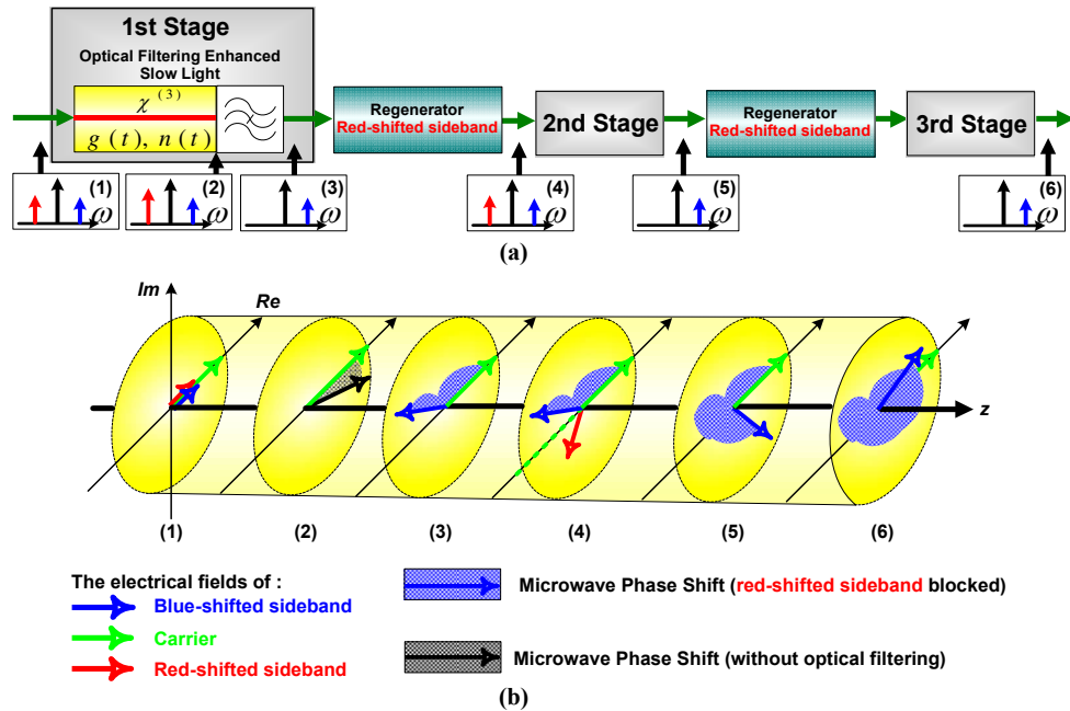
Fig. 1. Configuration of a 360^\circ microwave photonic phase shifter. (a) Simplified diagram showing the cascading of stages of phase shifters followed by regenerators. Both functionalities can be implemented in active waveguides by using the effects of population oscillations and wave mixing. (b) Illustrations of the evolution of the complex amplitudes of the sidebands in a polar representation.
