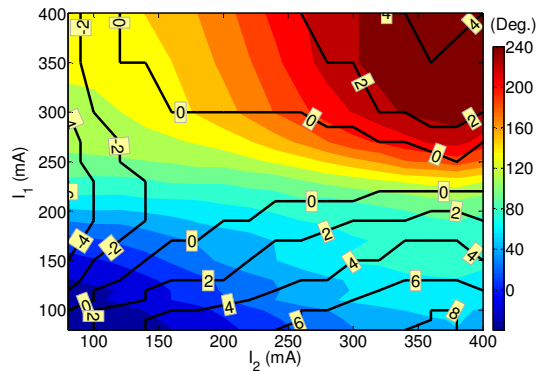
Fig. 5. Experimental demonstration of microwave phase shift (colour contour) and relative power change (black solid lines). The measurements are shown as a function of the currents I_1 and I_2 with I_3 being fixed at 80 mA, and performed at 40 GHz.
