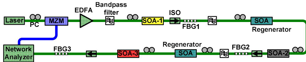
Fig. 3. Experimental set-up for measuring the microwave phase shift. (PC: polarization controller; MZM: Mach-Zehnder intensity modulator; EDFA: erbium doped fiber amplifier; ISO: fiber isolator; FBG: fiber Bragg grating). The laser at the wavelength of 1539nm is intensity modulated by the microwave electrical signal from the network analyzer, which is also used to measure the microwave phase shift induced by the SOAs.
