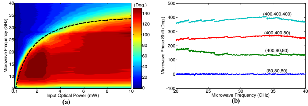
Fig. 6. Measured microwave frequency dependence of phase shifter. (a) Microwave phase shifts (colour scale) for a single phase shift stage as a function of microwave frequency and input optical power when blocking the red-shifted sideband. The black dashed curve shows the analytical result, Eq. (2). (b) Microwave phase shift for three cascaded phase shifter stages as a function of the microwave modulation frequency. The injection currents ( I_1 , I_2 , I_3 ) are consecutively increased from 80 mA to 400 mA.
