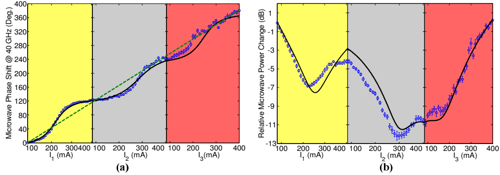
Fig. 4. Experimental demonstration of 360^\circ microwave phase shift. (a) Microwave phase shift and (b) power changes at the microwave frequency of 40 GHz. The injection currents ( I_1 , I_2 , I_3 ) are increased from 80 mA to 400 mA consecutively. The markers are experimental data and the black solid lines are numerical simulations. The green dashed line shows a linear fit.
