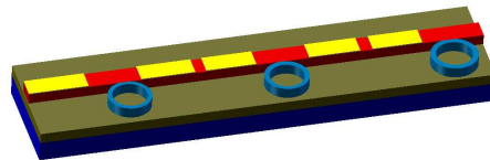
Fig. 7. Sketch of a possible monolithic implementation of a microwave photonic phase shifter with micro-rings to realize optical filtering.
