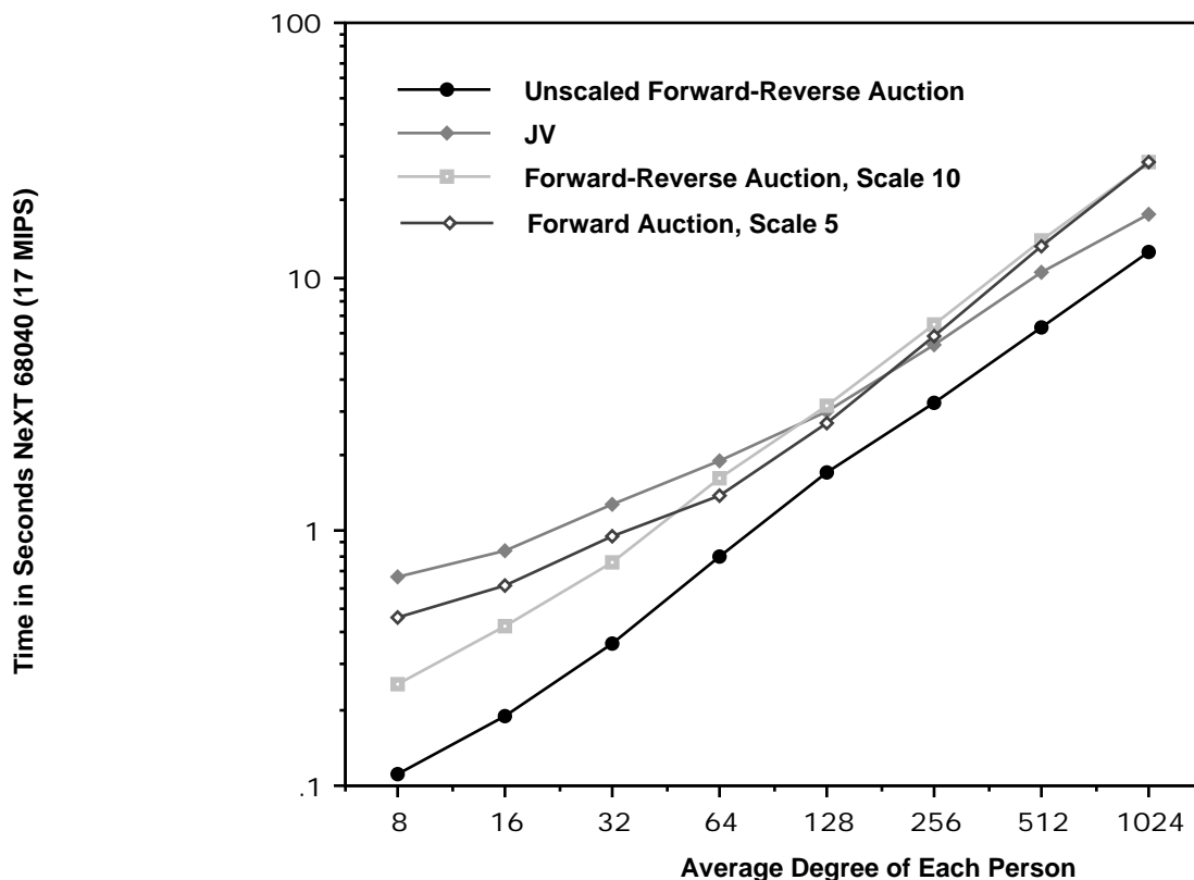
Figure 4: Run times for symmetric assignment problems on a NeXT 68040. The number of person nodes is 1024 and the average node degree varies. Each data point represents an average of thirty randomly generated problems. The arc benefits are drawn from the range [0,100000] according to a uniform distribution.
