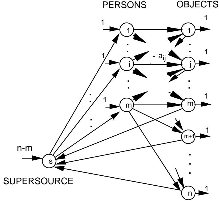
Figure 2: Converting a two-sided multiassignment problem into a minimum cost flow problem involving a supersource node s , zero cost artificial arcs (s, i) with feasible flow range [0, \infty) for each person i . and zero cost artificial arcs (j, s) with feasible flow range [0, \alpha_j - 1] for each object j .
