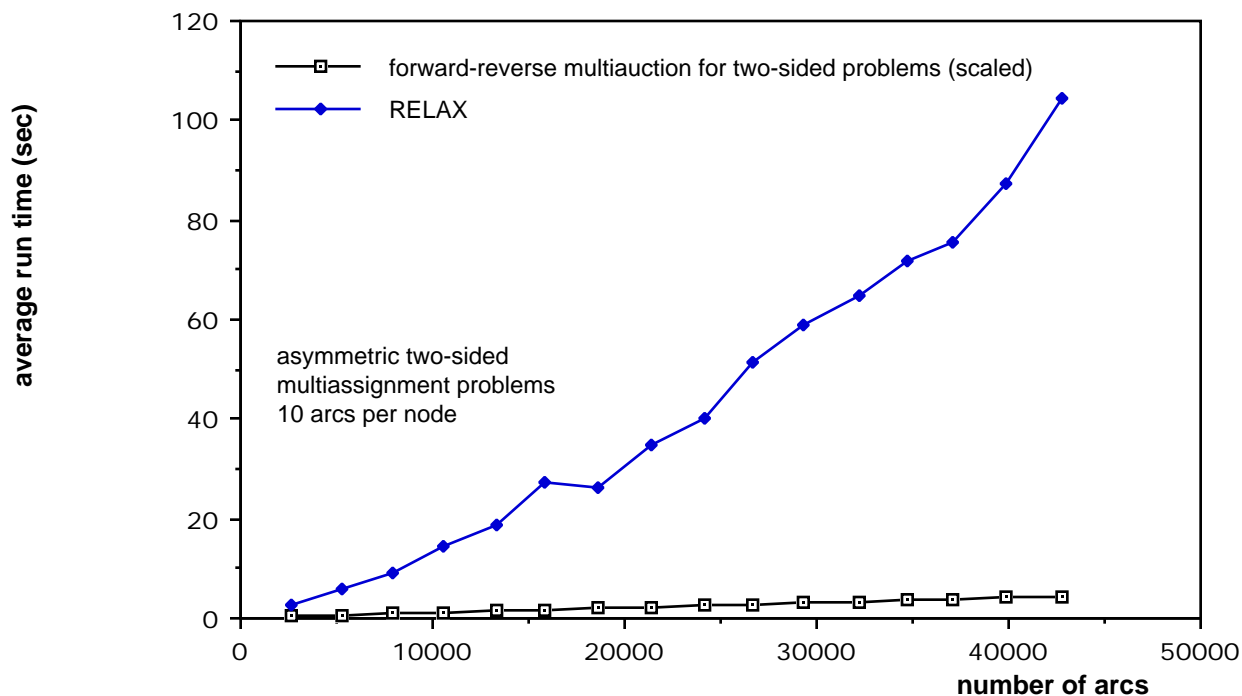
Figure 12: Run times for two-sided asymmetric multiassignment problems (cf. Eq. (43)) on a MAC II. The degree of each person node is 10 and the arc benefit range is [0,1000] . In these problems, the upper flow bounds \alpha_j are all \infty .
