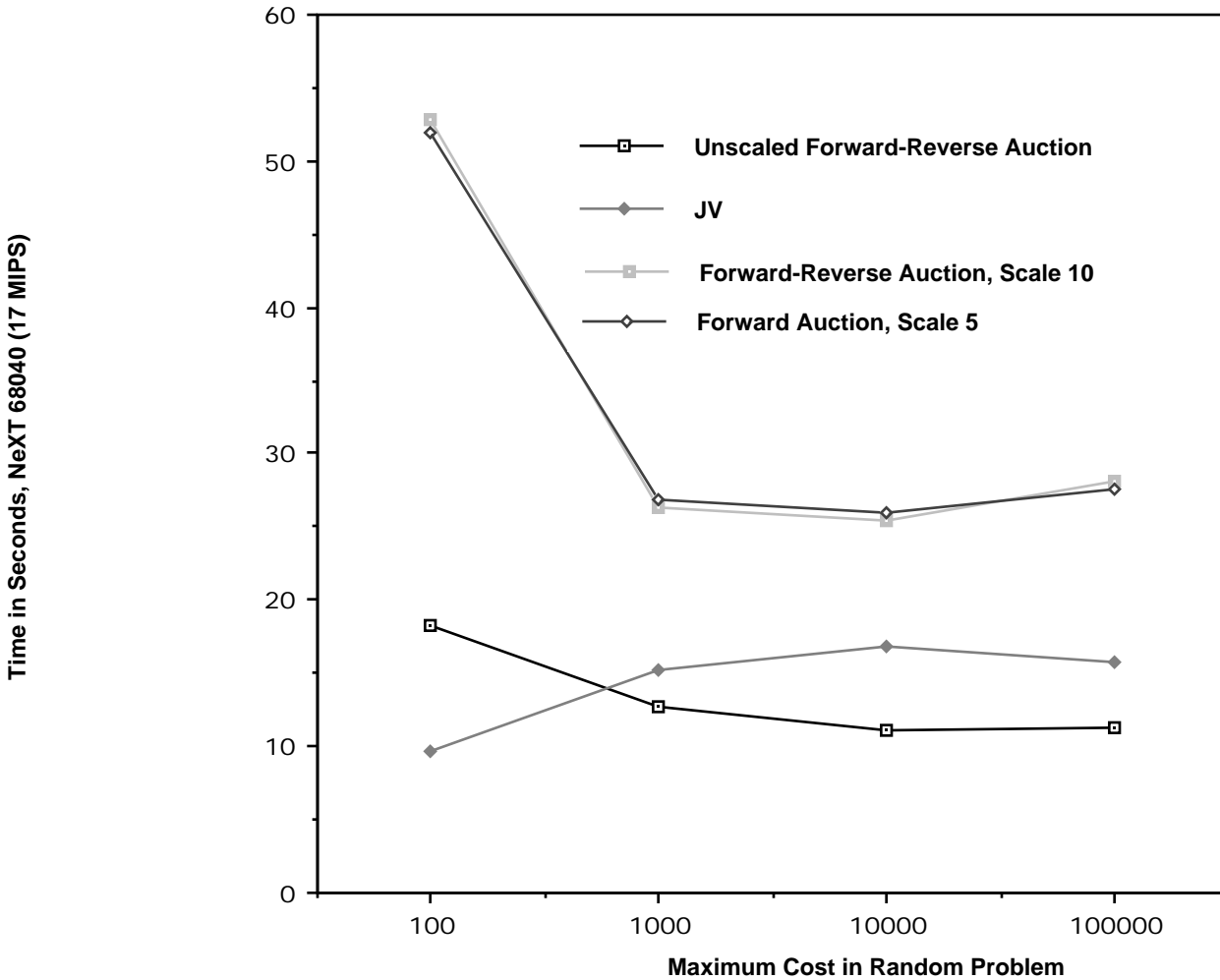
Figure 6: Run times for fully dense symmetric assignment problems with 1024 persons on a NeXT 68040. Each data point represents an average of thirty randomly generated problems. The arc benefits are drawn from the range indicated according to a uniform distribution.
