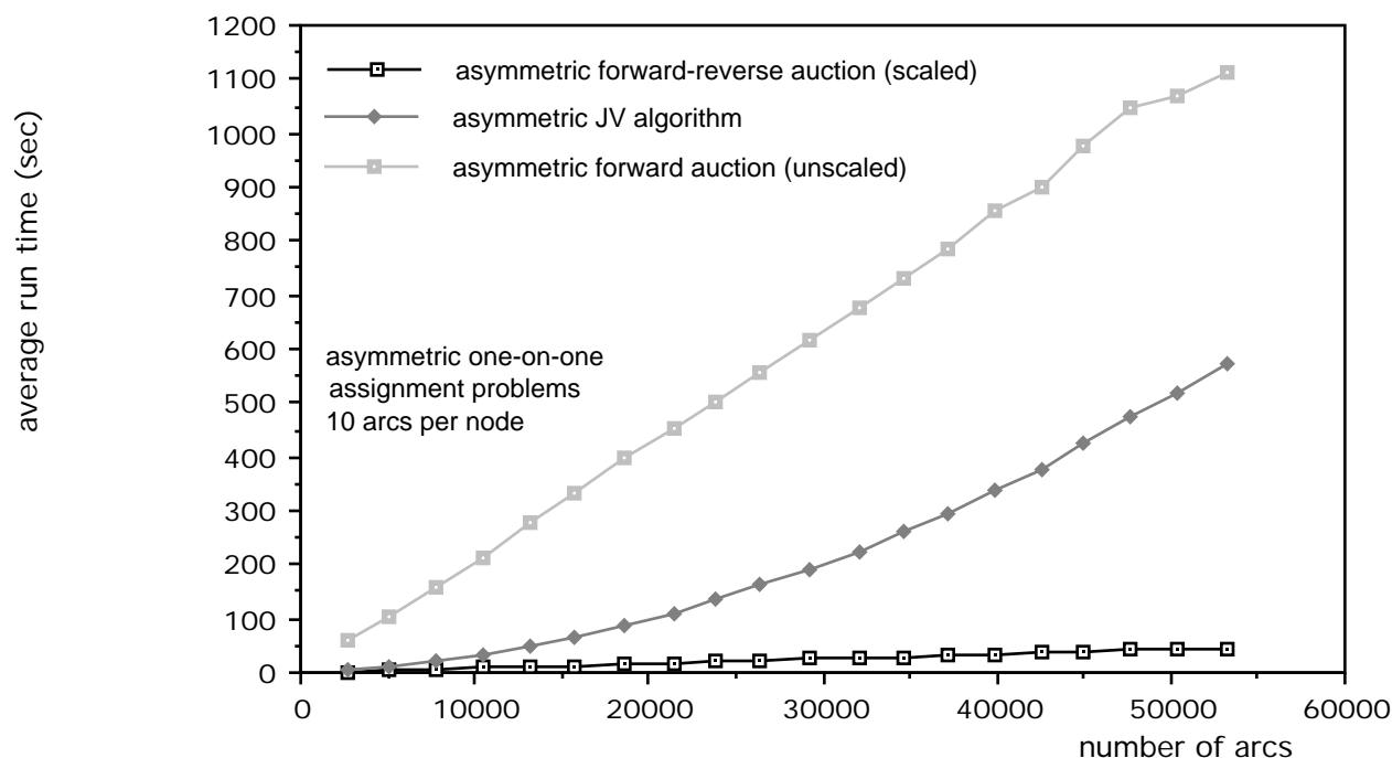
Figure 9: Run times for “difficult” asymmetric assignment problems on a MAC II. The degree of each person node is 10. Each data point represents an average of ten randomly generated problems. The standard deviation for each point was typically less than 5% of the corresponding run time. There are two levels of arc benefits that are different by approximately three orders of magnitude.
