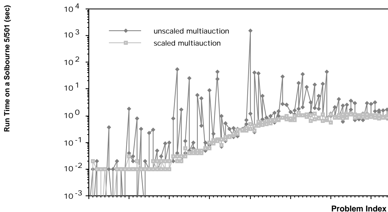
Figure 11: Run times for practical one-sided asymmetric multiassignment problems arising in multitarget tracking on a Solbourne 5/501 computer, rated at 22 MIPS. Each point on the horizontal axis corresponds to a different problem. The number of object nodes ranges from 10 to 125, and the number of arcs ranges from 100 to 10,000.
