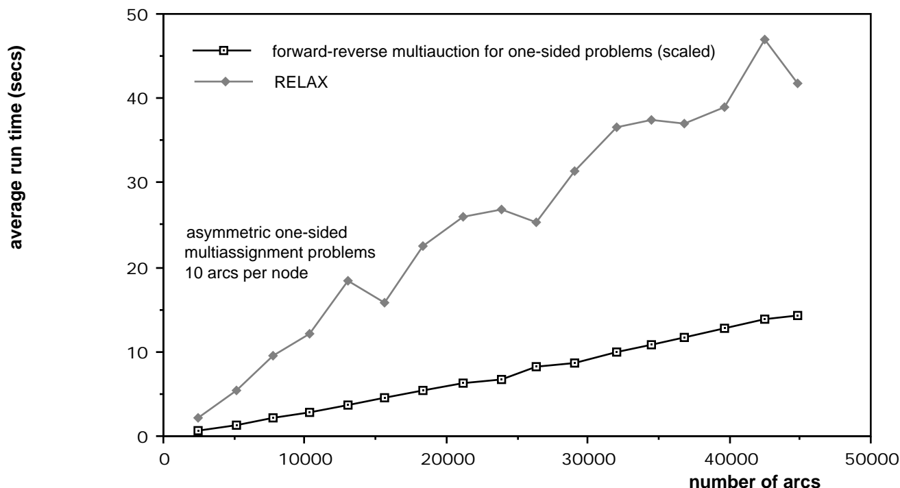
Figure 10: Run times for one-sided asymmetric multiassignment problems on a MAC II. Each data point represents an average of ten randomly generated problems. The degree of each person node is 10 and the arc benefit range is [0,1000] . The standard deviation for each point in the multiauction curve was typically around 5% of the corresponding run time, while for the RELAX curve it was between 10 and 30%.
