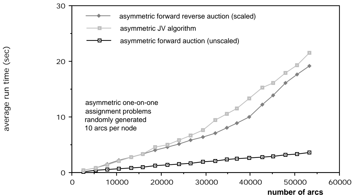
Figure 8: Run times for “easy” asymmetric assignment problems on a MAC II. The degree of each person node is 10 and the arc benefit range is [0,1000] . Each data point represents an average of ten randomly generated problems. The arc benefits are drawn from the benefit range according to a uniform distribution.
