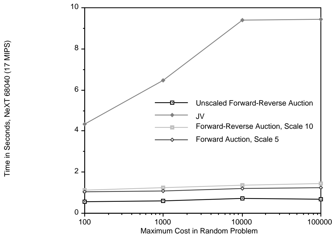
Figure 5: Run times for symmetric assignment problems on a NeXT 68040. The number of person nodes is 4000 and the degree of each is 8. Each data point represents an average of thirty randomly generated problems. The arc benefits are drawn from the range indicated according to a uniform distribution.
