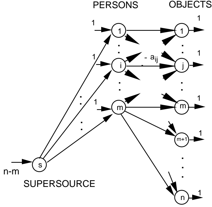
Figure 1: Converting a multiassignment problem into a minimum cost flow problem involving a supersource node s and a zero cost artificial arc (s, i) with feasible flow range [0, \infty) for each person i .
