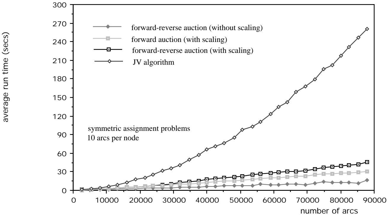
Figure 3: Run times for symmetric assignment problems on a MAC II. The degree of each person node is 10. Each data point represents an average of ten randomly generated problems. The arc benefits are drawn from the range [0,1000] according to a uniform distribution.
