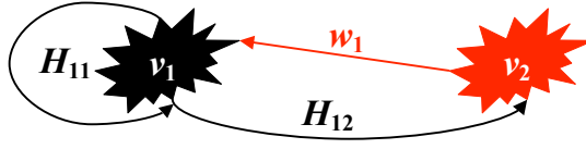
FIG. 4.3. Sources of PageRank when w_2 = 0 . The dangling nodes receive their PageRank only from v_2 , and from the PageRank of the nondangling nodes, filtered through the links H_{12} .
