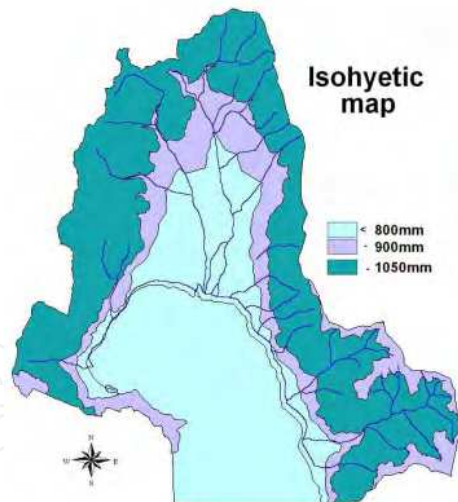
Fig. 9. Climatic types and isohyetic map of Macro Prespa Lake (Macedonian part only).
