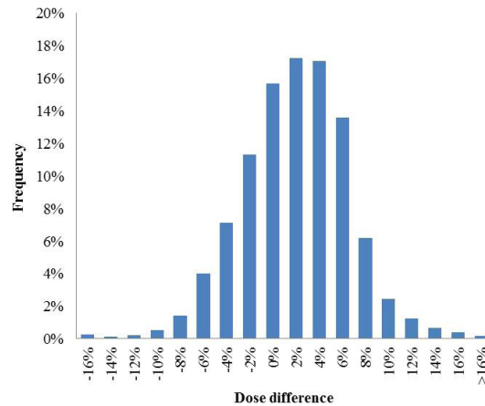
FIG. 4. Dose difference distribution of the IVD results for the period of July 2013 to June 2015.
