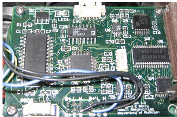
Fig. 19. Drive Motor Controller Board.
