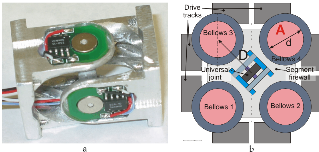
Fig. 13. a – Outer universal joint, with Hall-effect joint angle sensor. b – Cross-section of the Integrated Joint Actuator.
