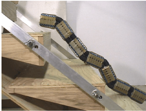
Fig. 7. Joint strength and stiffness: OT-4 lifting up three lead segments in order to reach the next step.
