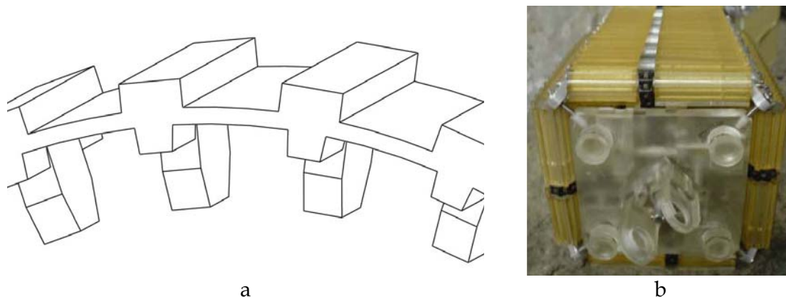
Fig. 10. a - Profile of the OT-8's urethane tracks, b - Front view of the OT-4. The extra-wide track areas add stability and reduce the risk of rollovers.
