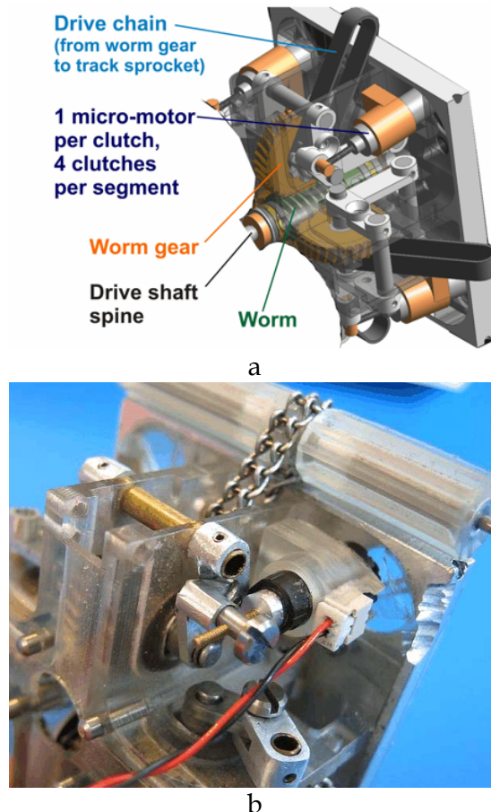
Fig. 26. Gear box and micro-clutches. a - CAD drawing, b - photograph
