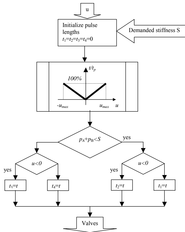
Fig. 16. Flow chart for the valve control subsystem.
