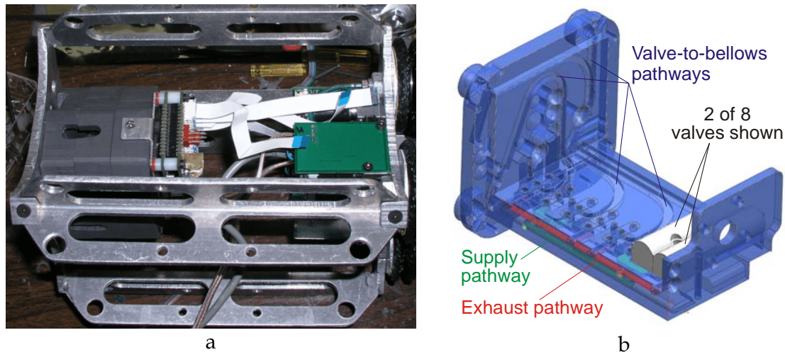
Fig. 12. a – Aluminum frame of the OT-8 with gearbox, controller boards and manifolds with white flat cables visible inside, b – Manifold of the OT-4 with two of the eight valves (white) mounted. Exhaust and supply pathways from and to the bellows are shown in red and green, respectively. This manifold is also partially the chassis of the six OT-4 actuation segments.
