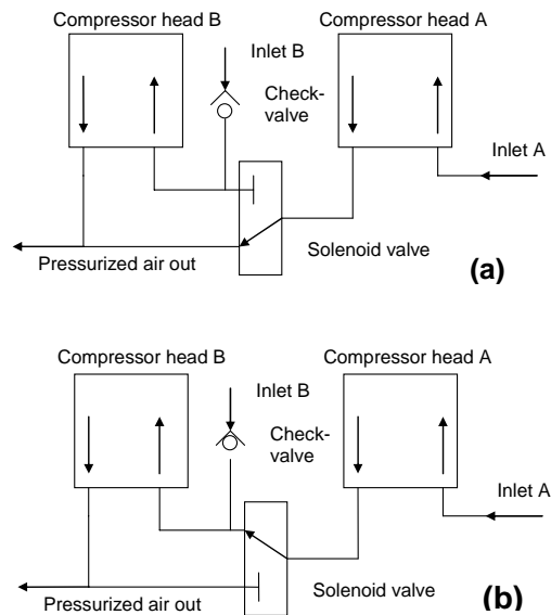
Fig. 21. (above) Modified dual-head air compressor installed in Segments #2 and #6.
