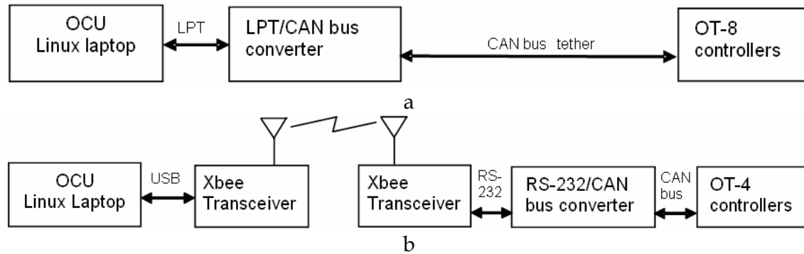
Fig. 24. Control communication system components. a – tethered system for OT-8. b – wireless system for OT-4.
