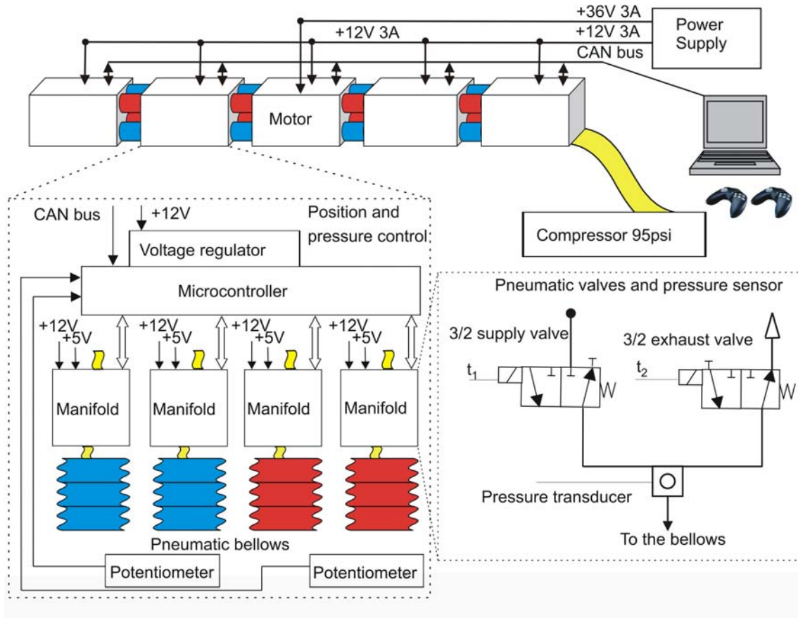
Fig. 17. Schematic diagram of the OmniTread control system, shown for the OT-8.
