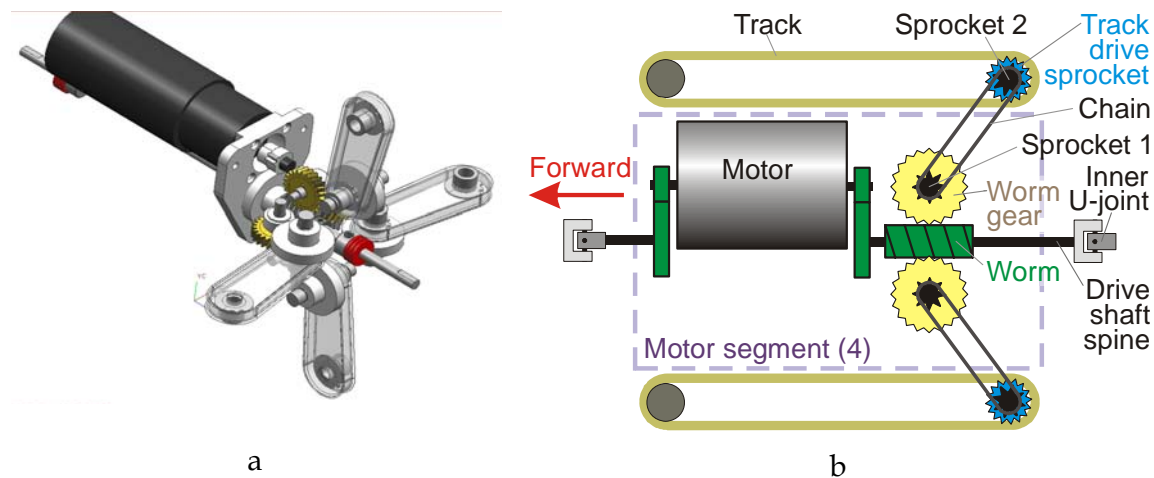
Fig. 9. CAD drawings of the OmniTread gearboxes: a - OT-8 gearbox, shown here for the motor segment. b - Schematic of the OT-4 drive system, shown here for the motor segment. c - CAD drawing of the OT-4 motor segment.
