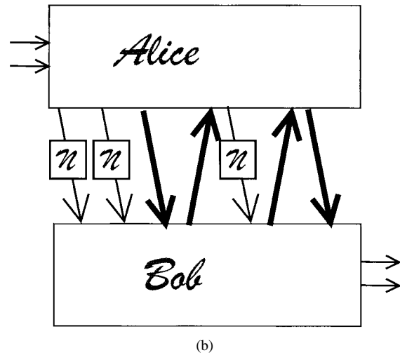
Fig. 3. (a) Unassisted quantum capacity Q of a noisy quantum channel is defined by the asymptotic performance of quantum error-correcting codes. (b) Classically assisted quantum capacity Q_2 is defined by the asymptotic performance of protocols involving forward uses of the noisy channel and unlimited classical communication between sender and receiver.
