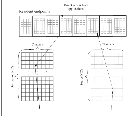
Figure 4: NIC channel tables. The NIC channel tables provide easy-access to NIC flow control, timeout/retry, and error detection information. The NIC uses stop-and-wait flow control on each channel and manages communication state information in channel table entries. In the send table (left), each entry includes timeout/retry information (packet timestamp, pointer to an unacknowledged packet, number of retries with no receiver feedback), sequencing information (next sequence number to use), and whether the entry is in use or not. In the receive table (right), each entry contains sequencing information for incoming packets (expected sequence number). Half of the channels are reserved for requests; the other half is reserved for replies. This is necessary in order to prevent deadlock.
