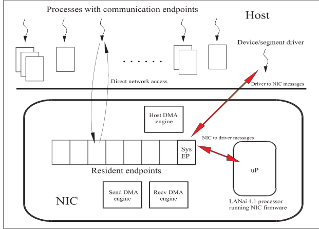
Figure 1: Processor/NIC node.
