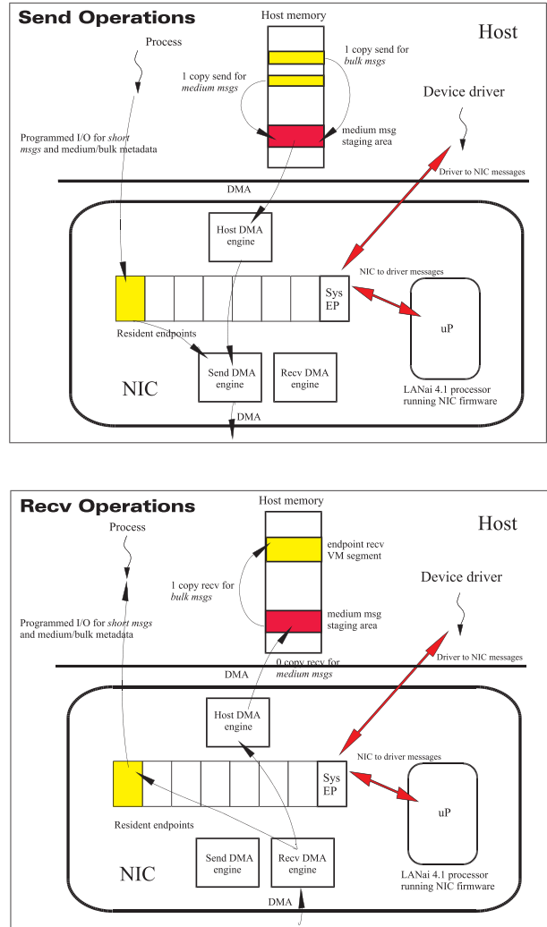
Figure 2: Data paths for sending and receiving short, medium, and bulk active messages. Short messages are transferred using programmed I/O directly on endpoints in NIC memory. Medium messages are sent and received using per-endpoint medium message staging areas in the pageable kernel heap that are mapped into a process's address space. A medium message is a single-copy operation at the sending host and a zero-copy operation at the receiving host. Bulk memory transfers, currently built using medium messages, are single-copy operations on the sender and single-copy operations on the receiver.
