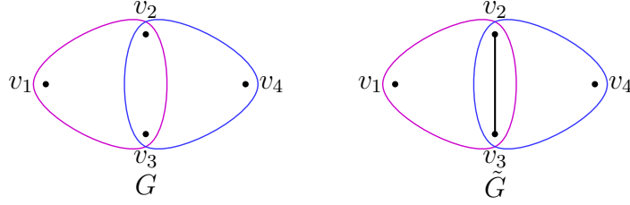
Figure 2: The hypergraphs G and \tilde{G} of Example 2 demonstrating that in certain cases, the inducing assumption of Theorem 2 can be relaxed.
