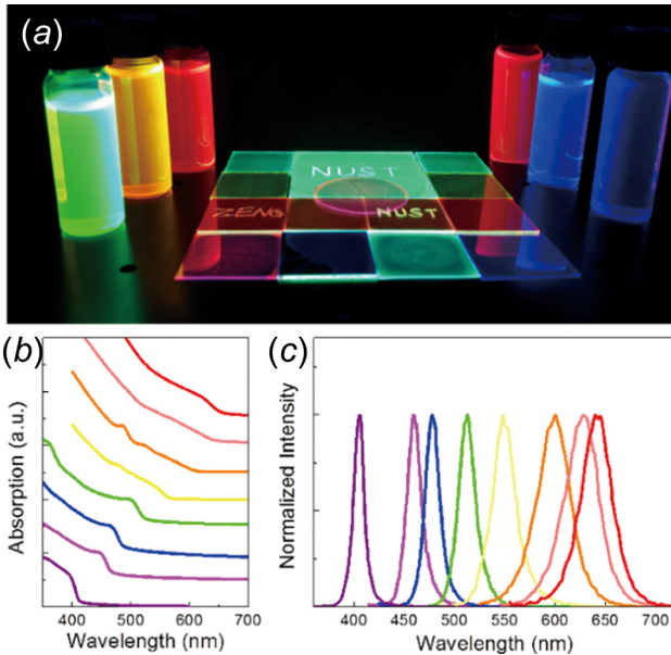
Fig. 1 (a) Composition-dependent change of the emission color from colloidal solutions of all-inorganic perovskite cesium lead halide ( \text{CsPbX}_3 , X = \text{Cl}, \text{Br}, \text{I} ). (b) Optical absorption and (c) PL spectra of colloidal \text{CsPbX}_3 QDs [17].
