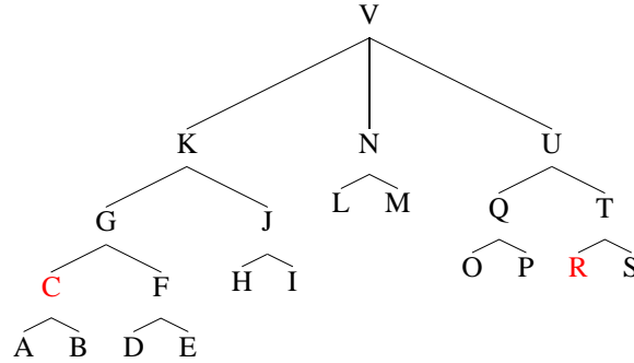
Figure 2. Example tree for the second case.
