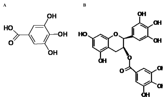
Figure 1. Structure of gallic acid (GA) (A) and epigallocatechin gallate (EGCG) (B).
