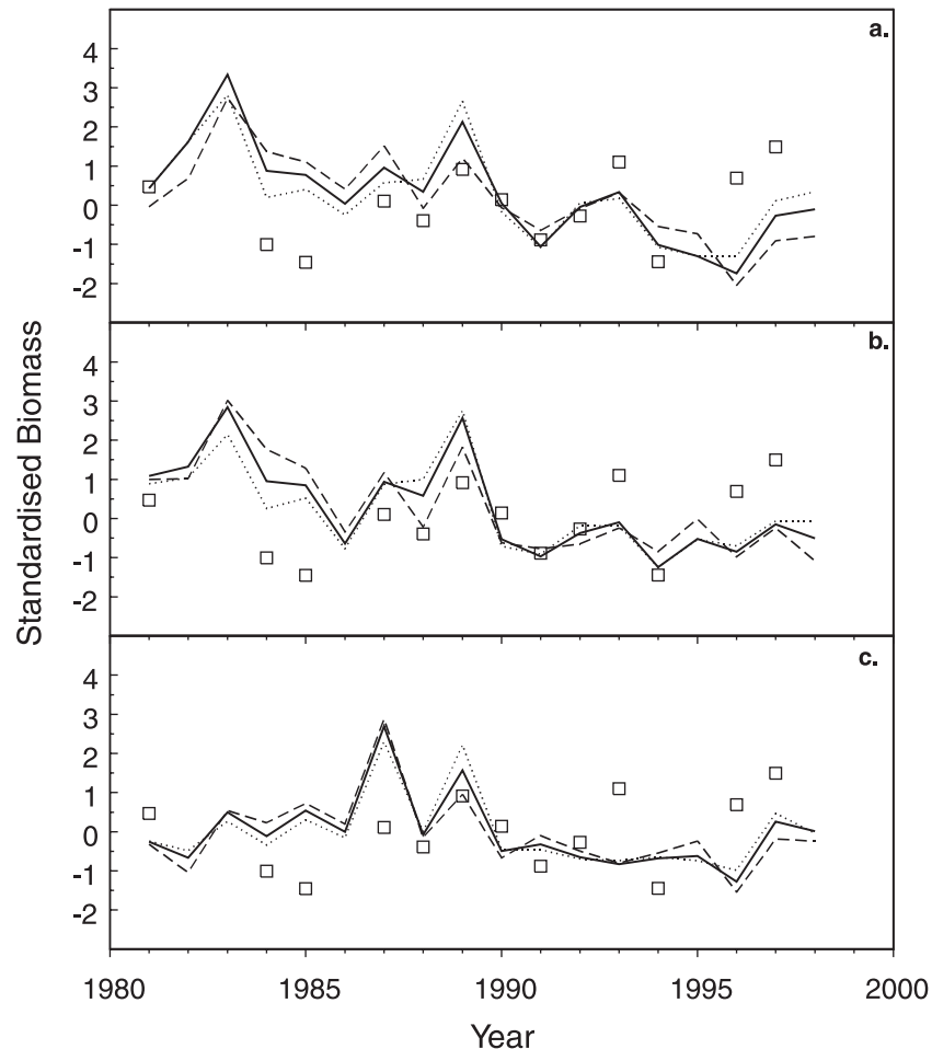
Figure 8. Standardized biomass densities for Elephant Island from simulations comparing model outputs with the acoustic time series, following Figure 7b. Sensitivity of the models to different rates of average annual natural mortality: (a) model with interannual variation in recruitment and interannual variation in mortality, (b) model with constant recruitment and interannual variation in mortality, and (c) model with constant mortality and interannual variation in recruitment. Open squares are observations from acoustic surveys. Solid lines, M = 0.8 ; dashed lines, M = 0.4 ; dotted lines, M = 1.2 .
