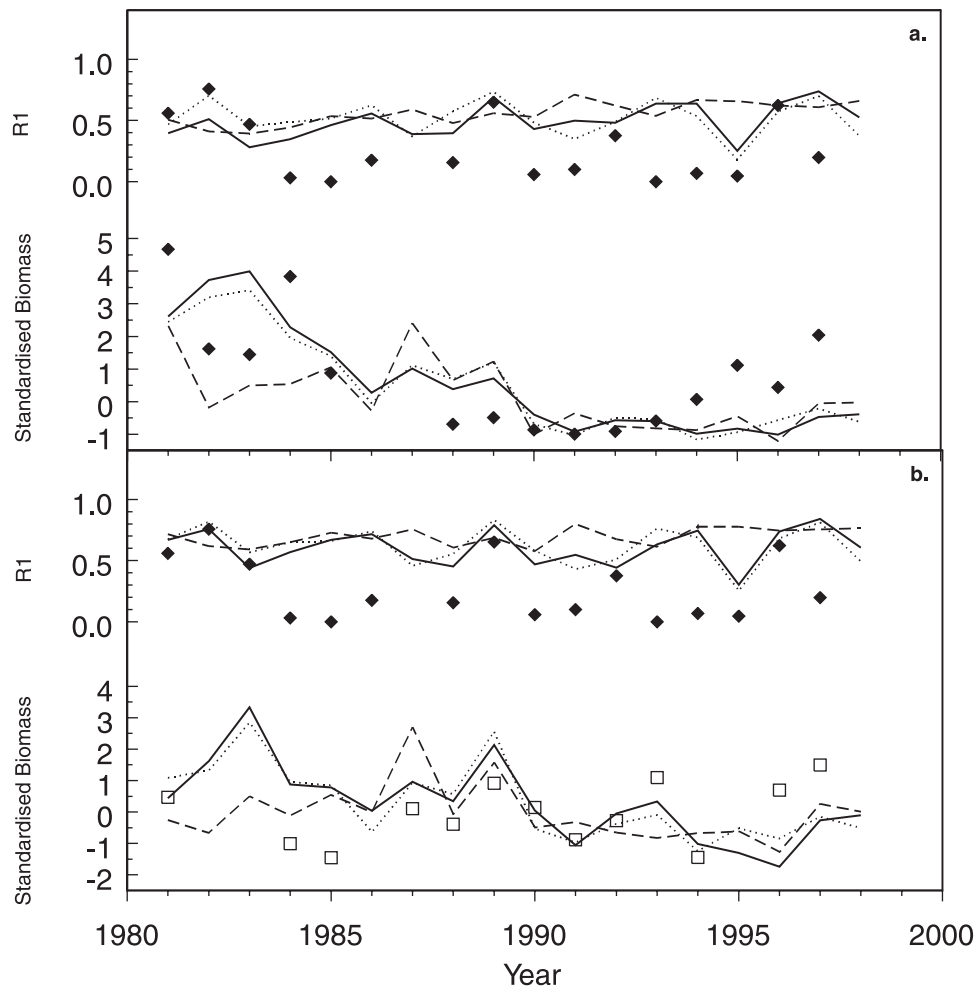
Figure 7. Standardized biomass densities and recruitment strengths (R1) for Elephant Island from model simulations using the recruitment and mortality time series shown in Figure 6 and fitting the time series to (a) the net-haul time series and (b) the acoustic time series. Fits were made by adjusting the migration patterns from the western Antarctic Peninsula and Weddell Sea into the Elephant Island area coupled with emigration from the area. Filled diamonds are observations from net-haul surveys. Open squares are observations from acoustic surveys. Solid lines are model with interannual variation in both recruitment and mortality. Dotted line is model with constant recruitment and interannual variation in mortality. Dashed line is model with constant mortality and interannual variation in recruitment.
