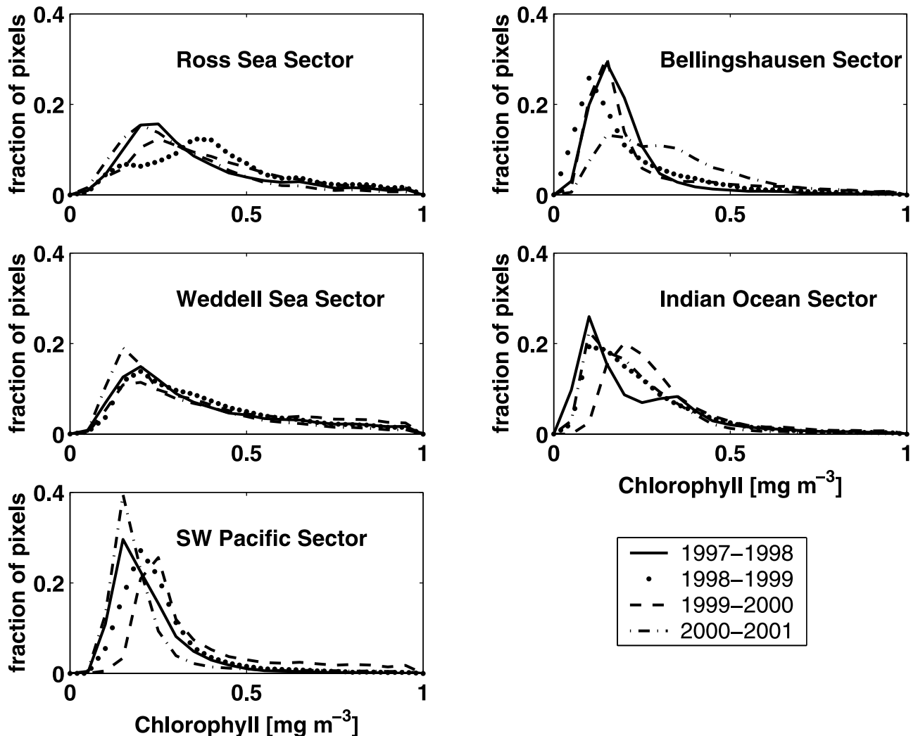
Figure 3. Frequency distribution of DJF SeaWiFS chlorophyll pixels in the five regions described above. Frequency distributions are quantified as a proportion (0–1) of all pixels in each region with chlorophyll <1.0 \text{ mg m}^{-3} .
