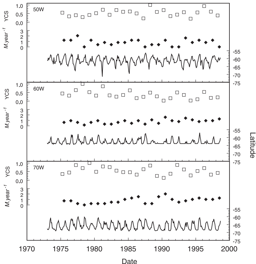
Figure 6. Ice extent (solid lines) at different longitudes: Weddell Sea (50°W), Elephant Island (60°W), and western Antarctic Peninsula (70°W) along with year class strength (YCS) (open squares) and mortality (filled diamonds) time series estimated from the ice data. Year class strength was translated directly to represent recruitment in the following year.
