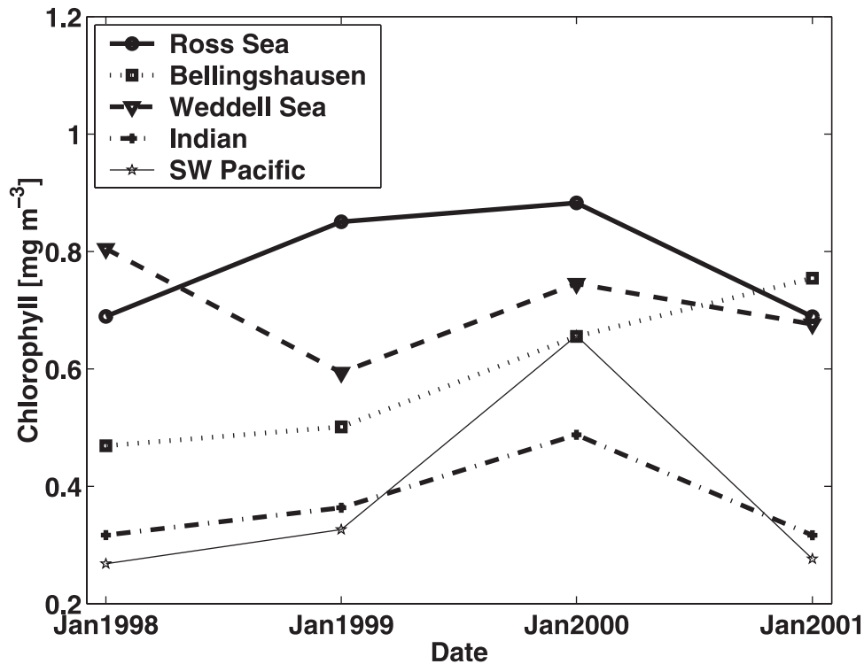
Figure 2. Mean DJF SeaWiFS chlorophyll concentration [ \text{mg m}^{-3} ] between the coast and PF in five regions defined by longitude [Arrigo et al. , 1998; Gloersen et al. , 1992]: The Ross Sea sector ( 160^{\circ}\text{E} to 130^{\circ}\text{W} ), the Bellingshausen/Amundsen Sea sector ( 130^{\circ} – 60^{\circ}\text{W} ), the Weddell Sea sector ( 60^{\circ}\text{W} to 20^{\circ}\text{E} ), the south Indian Ocean sector ( 20^{\circ} – 90^{\circ}\text{E} ), and the SW Pacific sector ( 90^{\circ} – 160^{\circ}\text{E} ).
