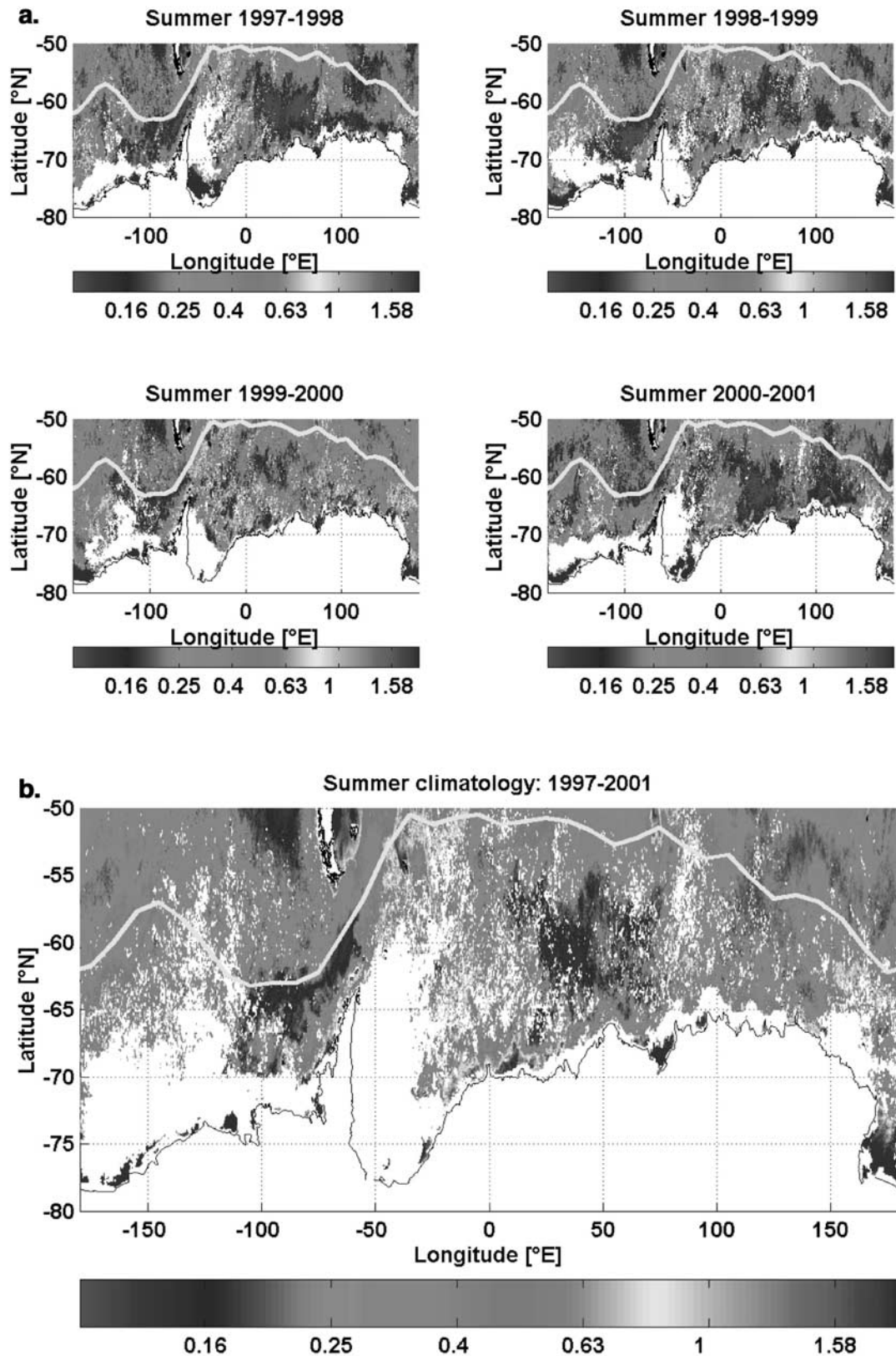
Figure 1. (a) Mean SeaWiFS chlorophyll concentration [ \text{mg m}^{-3} ] for the Austral summers (DJF) of 1997–1998, 1998–1999, 1999–2000, and 2000–2001. The PF, as described by Moore et al. [1999], is plotted in yellow. (b) SeaWiFS chlorophyll [ \text{mg m}^{-3} ] climatology for DJF 1997–2001. Mean chlorophyll was calculated using only pixels that contained valid data for all four summers depicted in Figure 1a. Color bar is chlorophyll [ \text{mg m}^{-3} ], and the PF is plotted in yellow.
