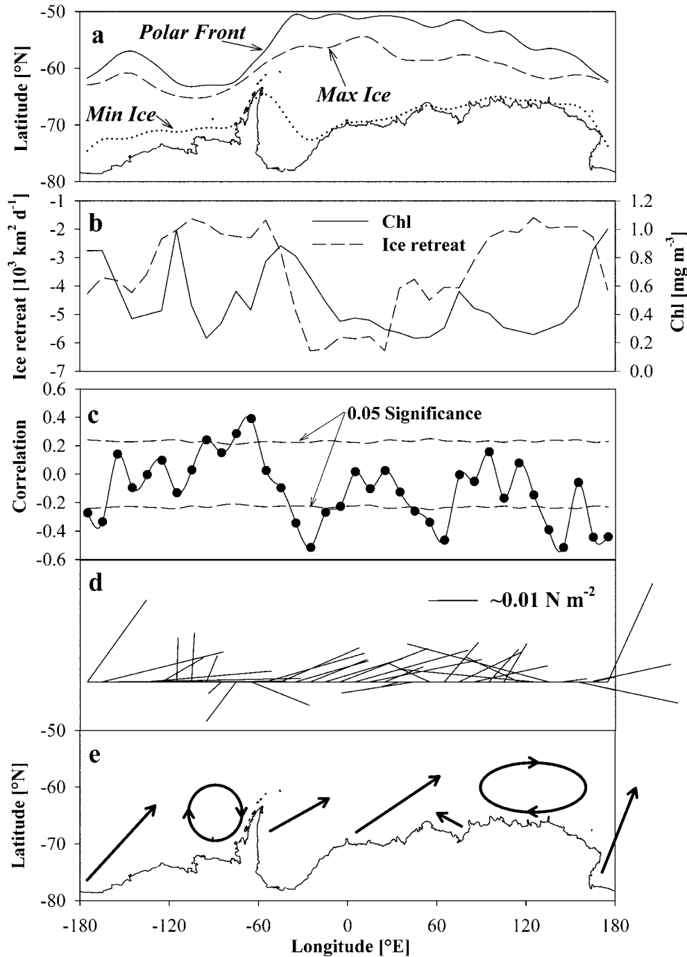
Figure 4. (a) The Antarctic coastline, the position of the PF (solid line), and the climatological maximum (dashed line) and minimum (dotted line) ice extent. (b) Mean DJF SeaWiFS chlorophyll concentration from 1997 to 2001 (solid line) compared to estimates of mean ice retreat (dashed line) as a function of longitude. (c) Correlation between rate of ice retreat and mean DJF SeaWiFS chlorophyll concentration as a function of longitude. A negative correlation implies that rapid ice retreat is correlated with high chlorophyll concentrations. The 0.05 significance level is plotted as a dashed line. The significance line is not straight because the number of observations varies as a function of longitude. (d) Climatological wind vectors, wind “sticks” point in the direction of the wind and the size of each stick is proportional to wind strength (scale indicates 0.01 \text{ N m}^{-2} ). (e) Representation of climatological winds around Antarctica as large-scale wind patterns.
