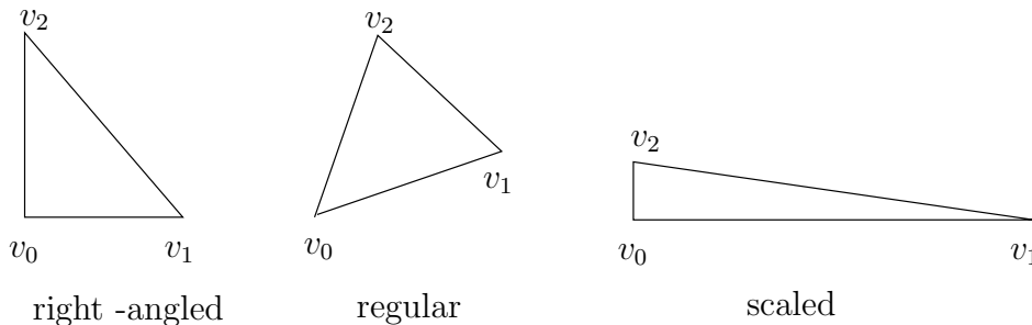
FIGURE 1: Selection of initial simplex
