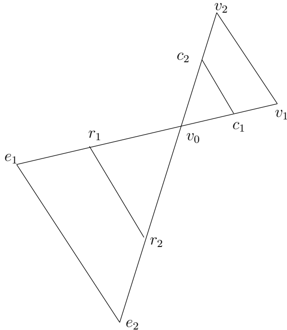
FIGURE 2: Reflection, expansion and contraction of current simplex
