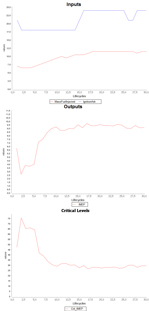
Figure 5: Controlling Injected Mass Fuel and Ignition Advance to Maximize IMEP
