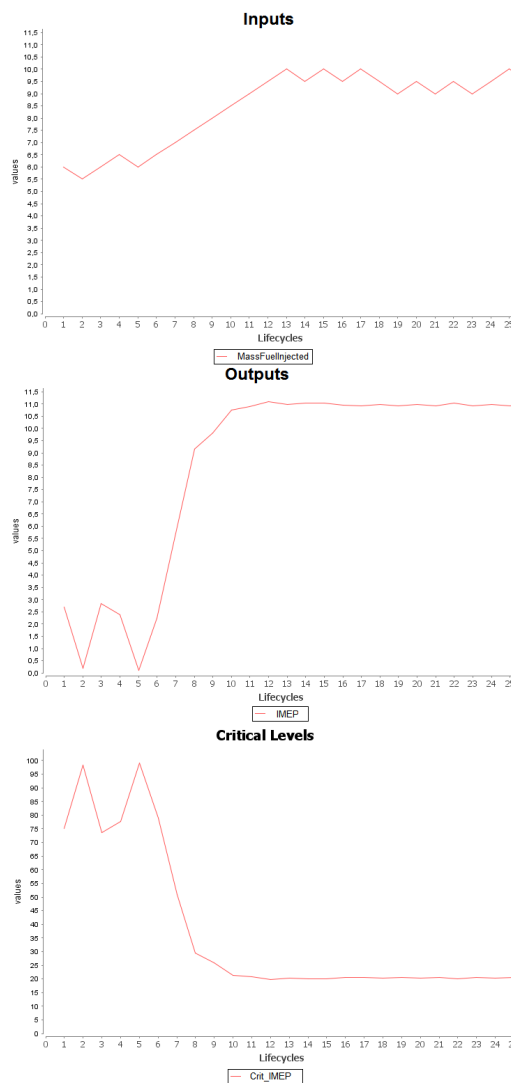
Figure 4: Controlling Injected Mass Fuel to Maximize IMEP
