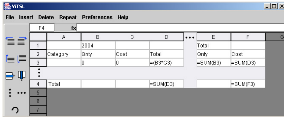
Figure 13: ViTSL interface.
