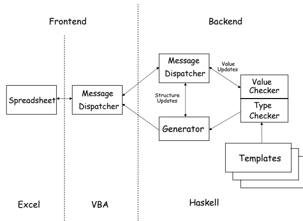
Figure 11: Gencil system architecture.
