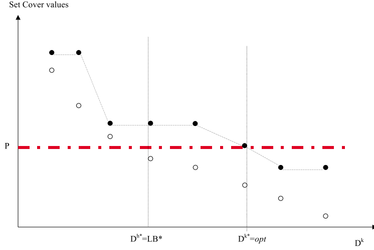
Figure 1: Illustration of h^* and k^* . \bullet : v(SC_{D^k}) , \circ : v(LSC_{D^k}) .
