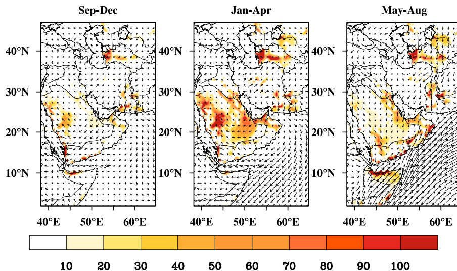
Figure 11. Climatology (seasonal average) of surface fine (0.01–1 μm) dust emission flux for fine dust (mg m -2 day -1 ) based on 2000–2012 interval.
