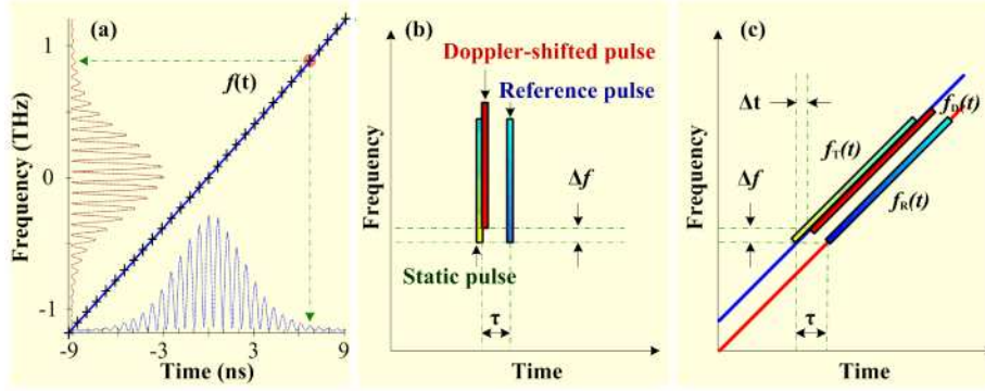
Fig. 2. Visualization of the instantaneous frequency on the frequency-time plane. (a) Time-to-frequency conversion function derived from the temporal and the spectral interferograms. (b) Femtosecond pulses before the dispersion. (c) Femtosecond pulses after the dispersion. To avoid pulse overlap, an offset perpendicular to the time-to-frequency conversion function is introduced between the Doppler-shifted pulse and the static pulse. One should also note that, generally, Doppler shift is very small relative to the optical bandwidth. For clarity, the Doppler shift is magnified in (b) and (c).
